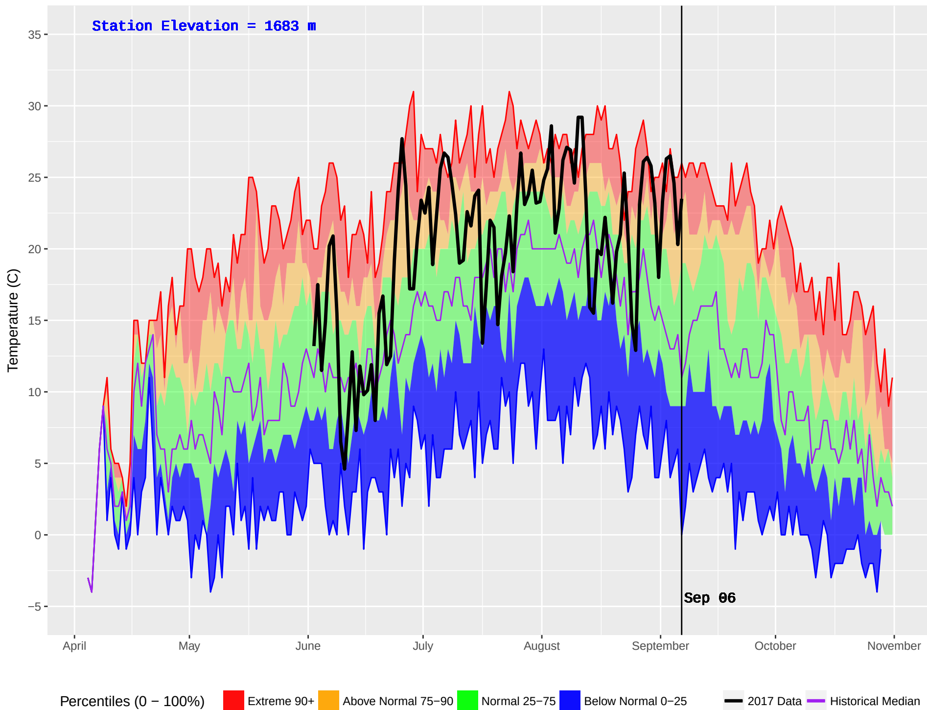
ASHNOLA (331) : Historical (1992–2016) and Current (2017) Noon Temperature
