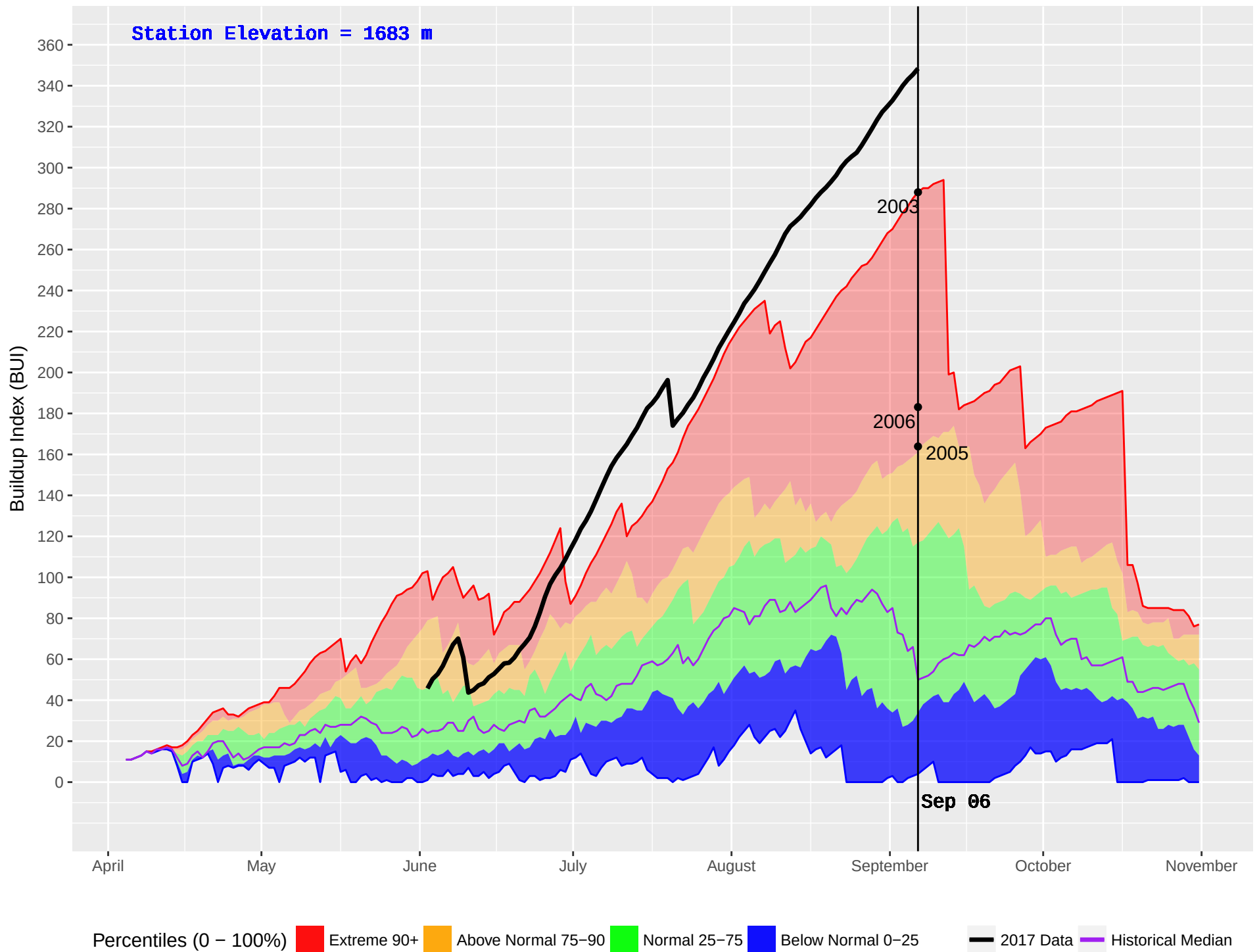
ASHNOLA (331) : Historical (1992–2016) and Current (2017) Noon Buildup Index (BUI)
